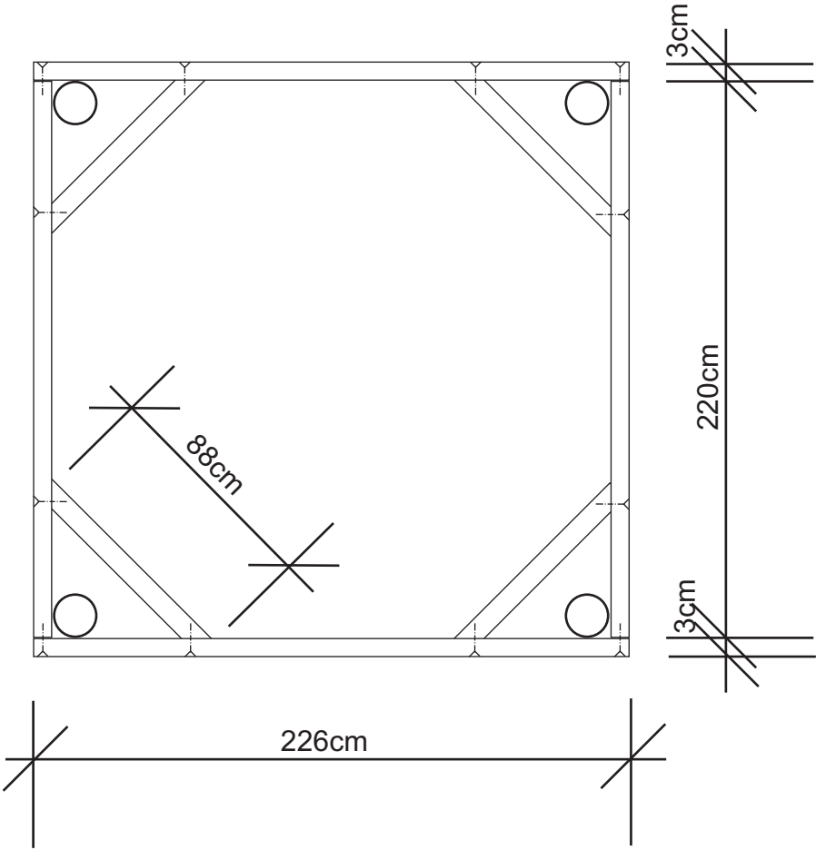
top view
