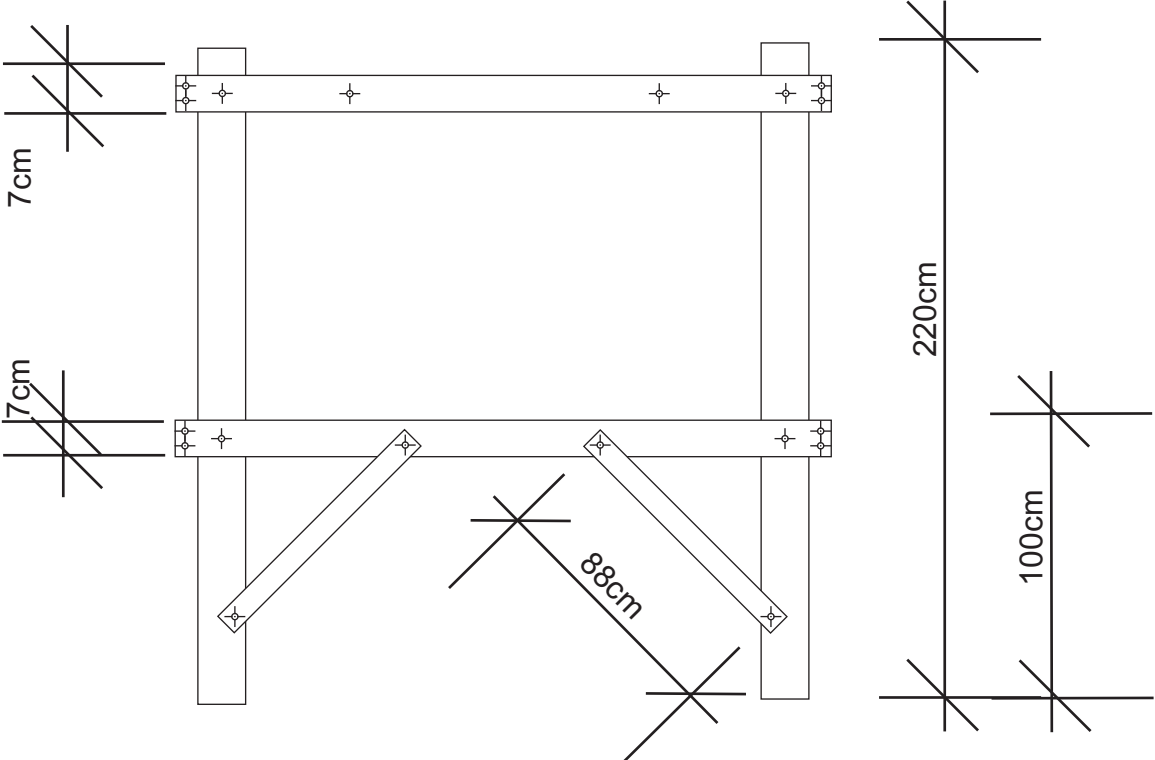
side view
